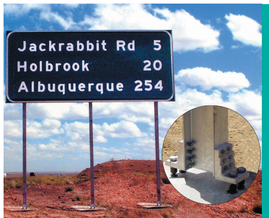
Figure 24. An Information Sign with Breakaway Supports (FHWA 2012f)
