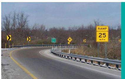
Figure 6. Example of Advisory Ramp Speed Sign and Chevrons (FHWA 2009b)
