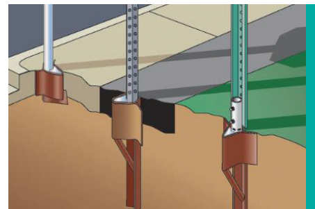
Figure 26. Sample of Breakaway Support System (Image: TAPCO)
